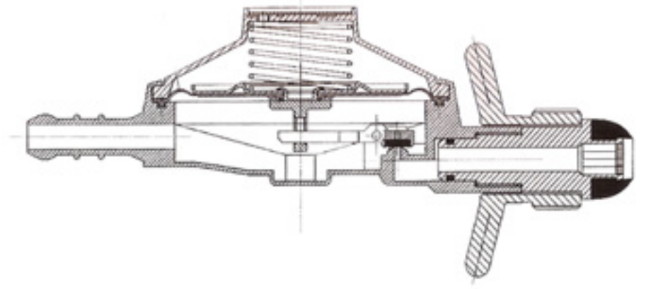
Threaded connect G1/4" LH - EN12.864 - H4
